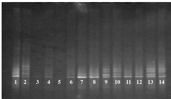
FIG. 3 : DGGE analysis of exon 9 of the LDL receptor gene. Lane 1 is a normal control, lane 2 a positive control (V408M mutation) whilst lanes 3 - 14 are samples of FH patients. Lanes 9, 10, 13 and 12 showed band shifts suggesting presence of mutations in these patients.
