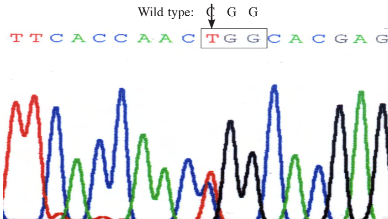
FIG. 6 : DNA sequencing results of exon 9 of the LDLR gene showing the base change from C → T at nucleotide 1216 resulting in substitution of amino acid arginine (R) to tryptophan (W) at codon 385, designated as R385W mutation.
