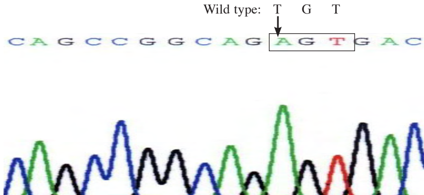
FIG. 5 : DNA sequencing results of exon 5 of the LDLR gene showing the base change from T → A at nucleotide 763 resulting in substitution of amino acid cysteine (C) to serine (S) at codon 234, designated as C234S mutation. This is an example of a homozygous mutation.
