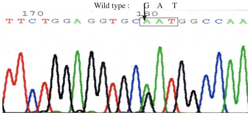
FIG. 4 : DNA sequencing results of exon 3 of the LDLR gene showing the base change from G → A at nucleotide 268 resulting in substitution of amino acid aspartic acid (D) to proline (N) at codon 69, designated as D69N mutation. This is an example of a heterozygous mutation (as demonstrated by two peaks).
