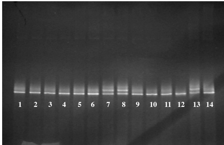
FIG. 2 : DGGE analysis of exon 5 of the LDL receptor gene. Lane 14 is the normal control, lane 13 the positive control with D245E mutation whilst lanes 1 - 12 are samples of FH patients. Lanes 7 and 8 show band shifts suggesting presence of mutations in this patient.
