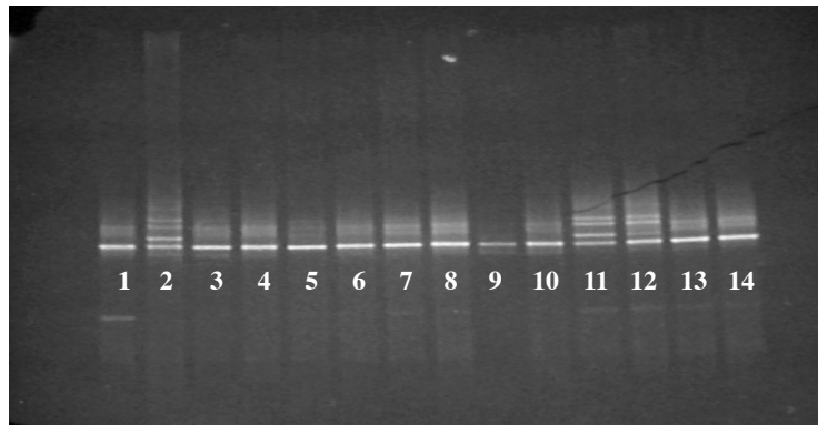
FIG. 1 : DGGE analysis of exon 3 of the LDL receptor gene. Lane 1 represents the normal control, lane 2 represents the positive control of R60C mutation, lanes 3 - 14 are samples of FH patients. Lanes 11 and 12 shows positive band shifts suggesting the presence of mutations
