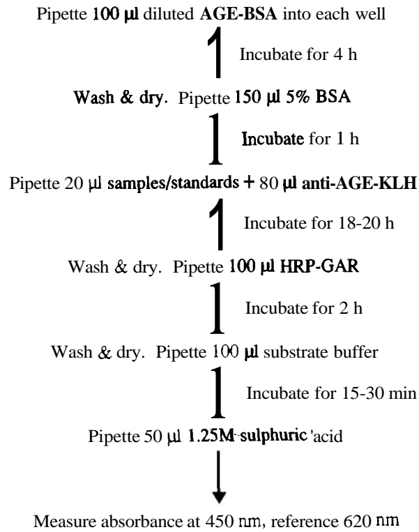
FIG. 1: Flow-chart for AGE EIA.
