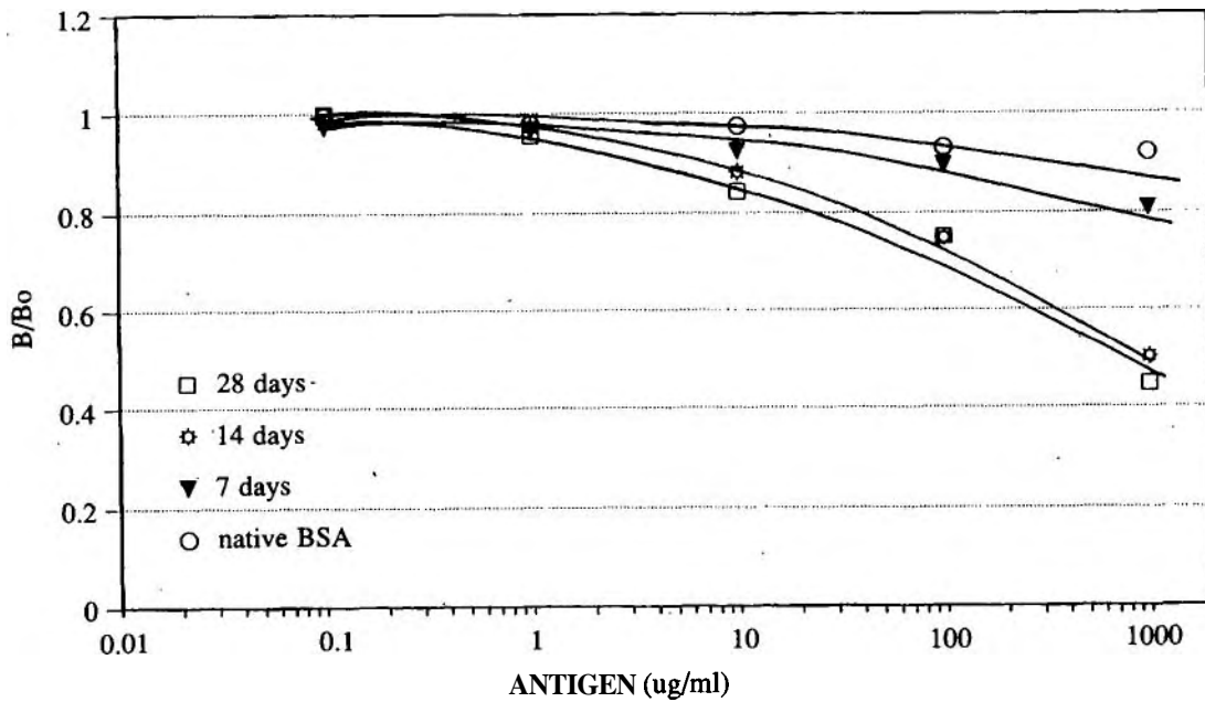
FIG. 2: Time-related increase in immunoreactivity of BSA incubated with glucose.
