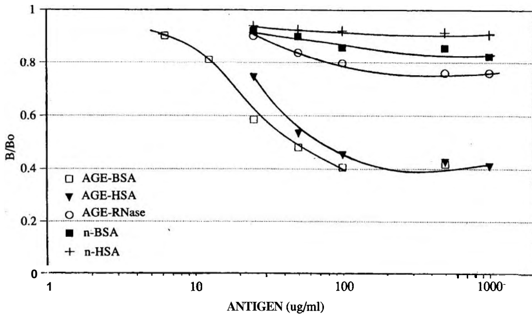
FIG. 4: Immunoreactivity curves of various AGE-proteins and related compounds with anti-AGE-KLH.
