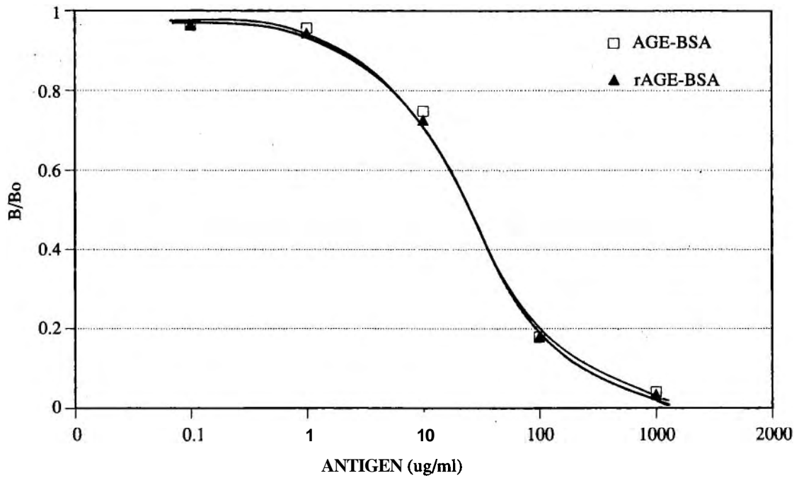
FIG. 3: Competitive EIA inhibition curves for AGE-BSA and chemically reduced AGE-BSA.
