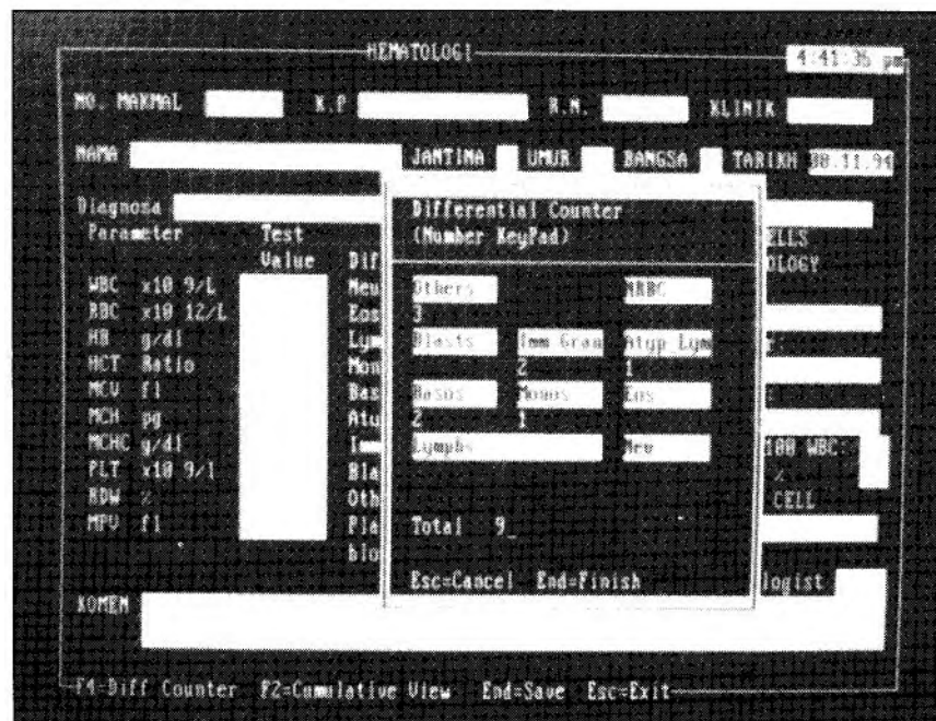
FIG. 4: The differential counter emulator appearing in a window superimposed on a data form display.
