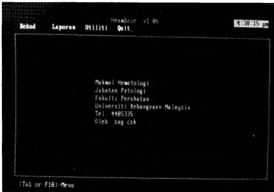
FIG. 2: The opening display of the software package. The horizontal menu bar is on top of the banner. Activation of an item in the menu bar produces further pull-down submenu.
